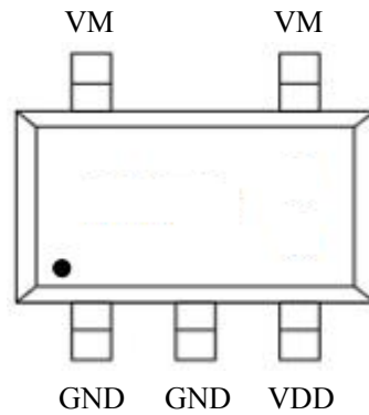
Figure 2. Pin Configuration
